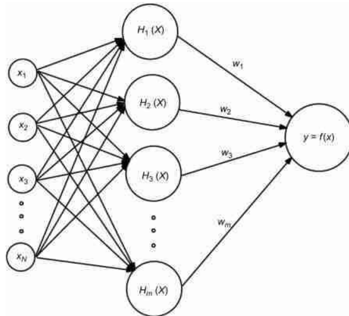
Figure 1. RBF Network Architecture
